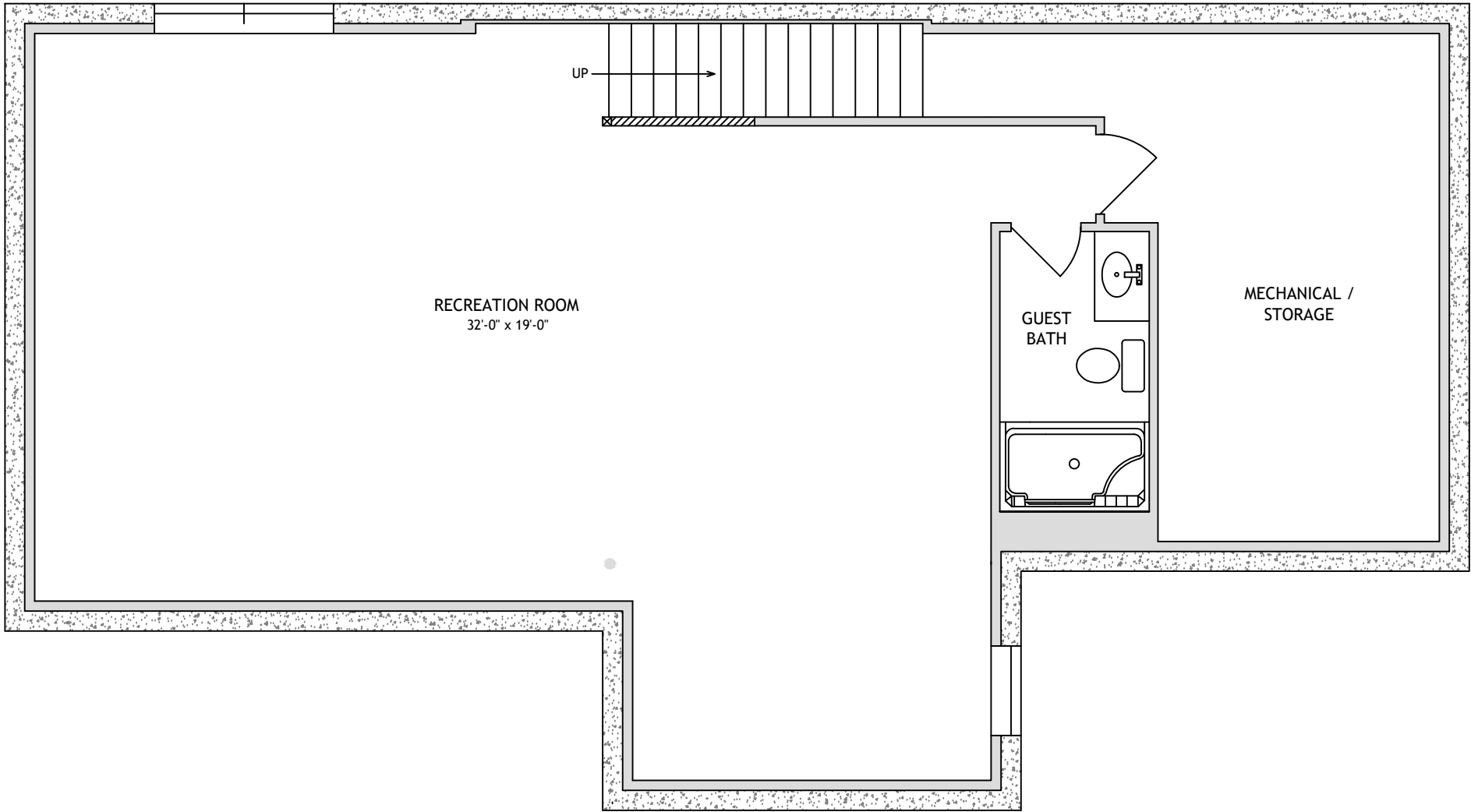
BASEMENT PLAN
